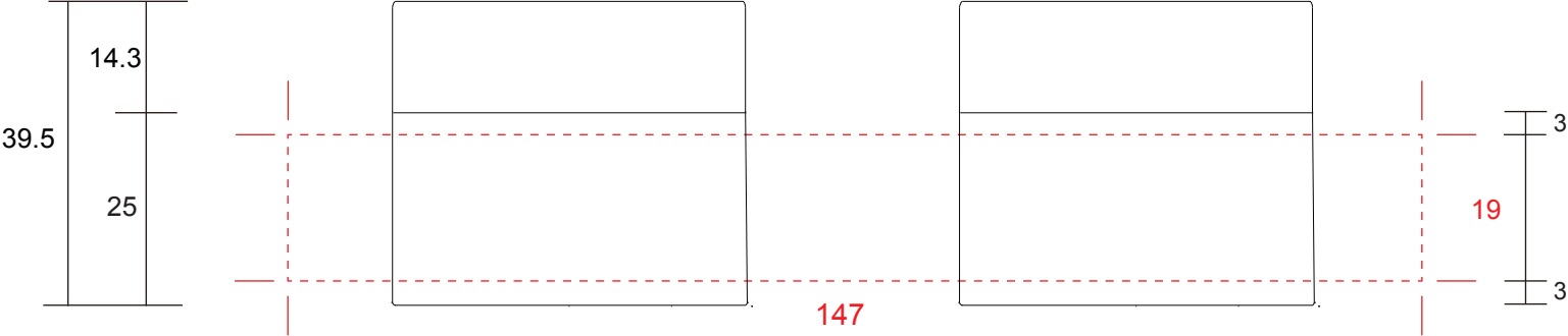
H-30B/ Jar Body
